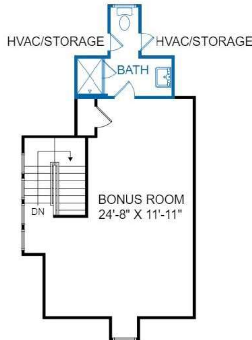
Loft Level Floorplan with options
