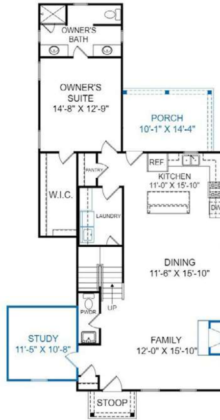
Main Level Floorplan with options
