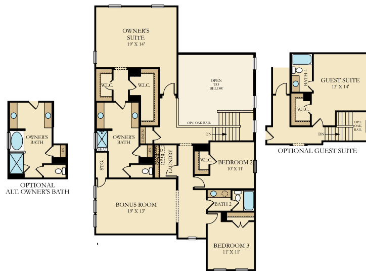
SECOND FLOOR
